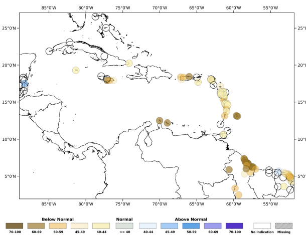
OND 2026 frequency of 7-day wet spells
