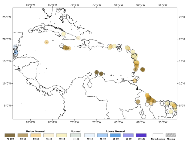
OND 2026 frequency of 7-day very wet spells
