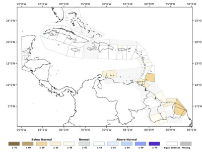
OND 2026 frequency of 7-day wet spells
