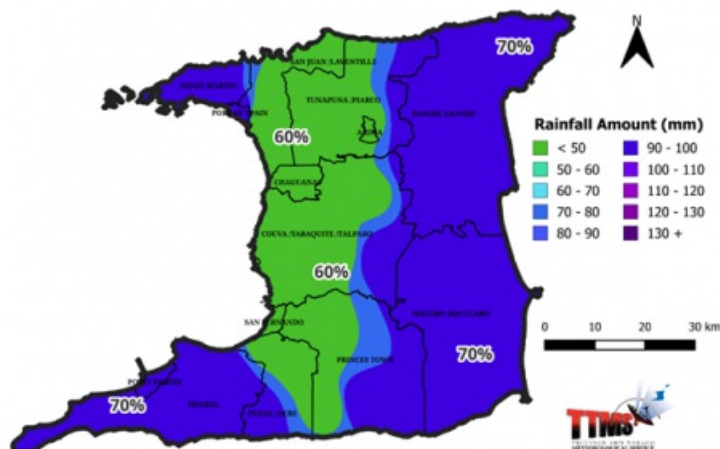
Figure 3. Rainfall map of Trinidad showing expected mean rainfall totals for districts across Trinidad during the 15-day period (1 st to 15 th August 2026) and percentage probability of occurrence.
