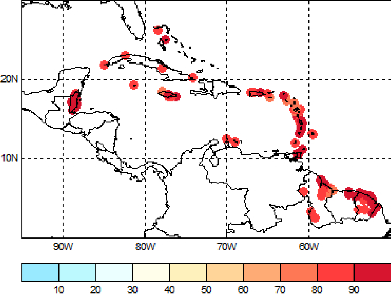
Prob. excessive rainfall event - Oct. to Dec. 2025
