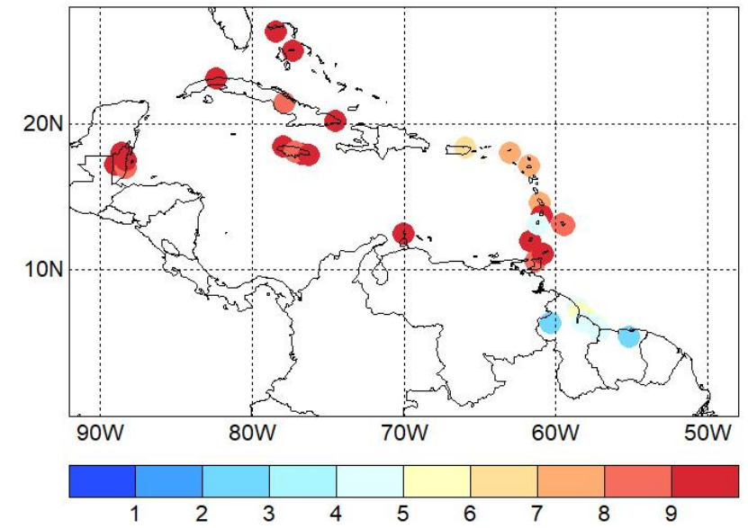
MAX number of 7-day dry spells
