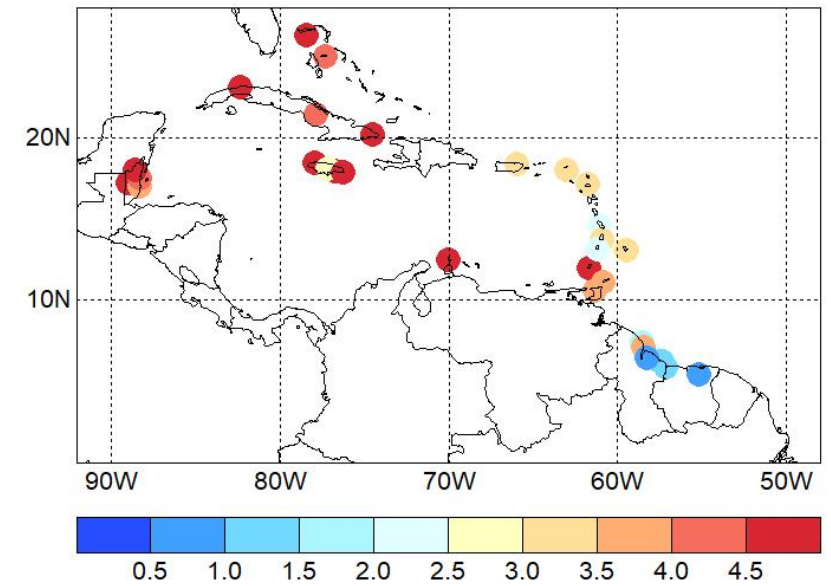
MAX number of 15-day dry spells
