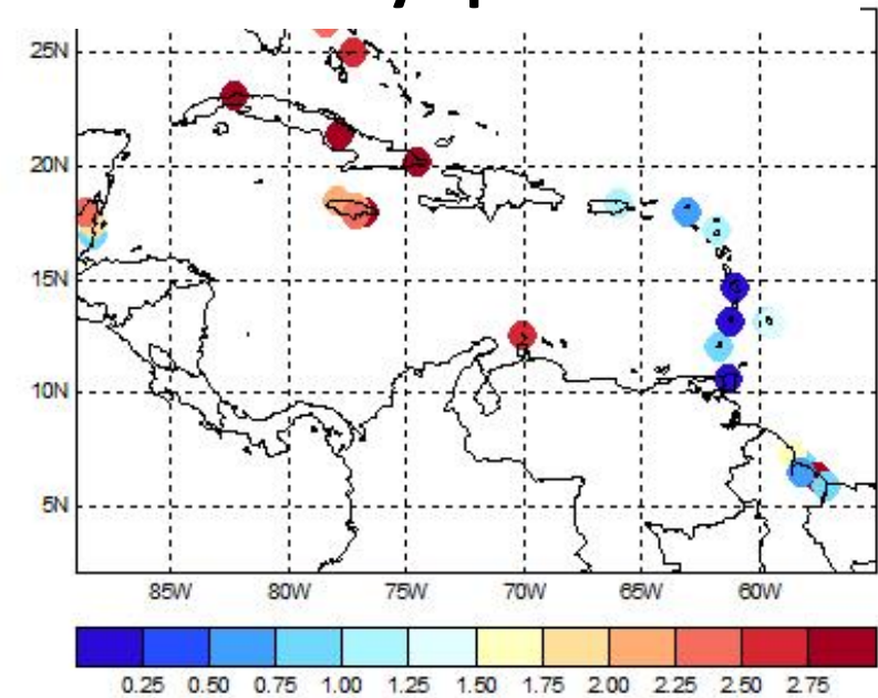
MAX number of 15-day dry spells
