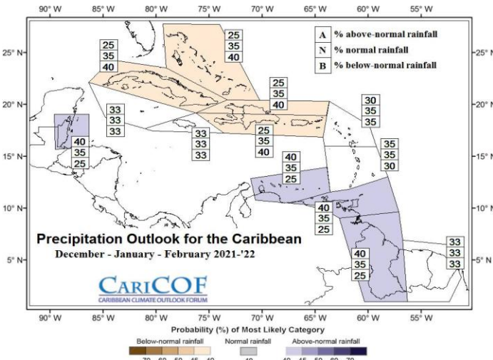
Fig 4. Regional Precipitation Outlook Dec-Jan-Feb 2021-22
