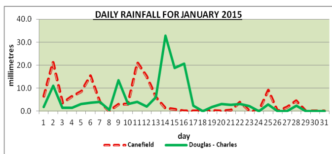
Figure 1 Daily rainfall at Canefield and Douglas-Charles Airports
