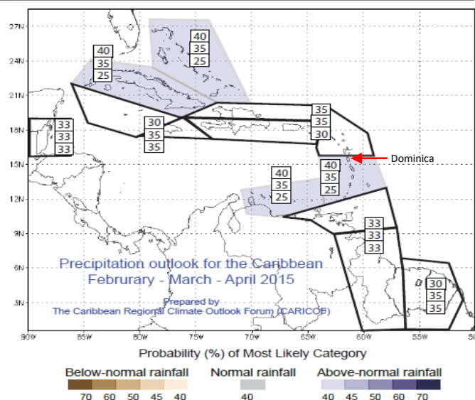
Figure 2 Precipitation outlook for the Caribbean: February-March-April 2015
